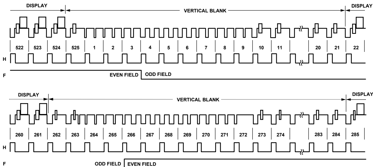
Figure 102. SD Master Mode 0, NTSC
