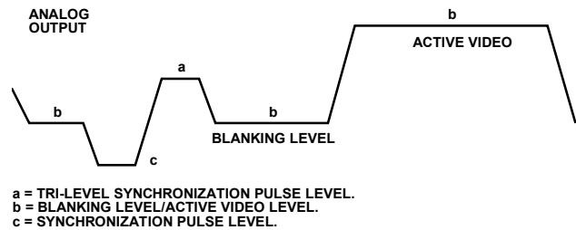
Figure 58. ED/HD Nonstandard Timing Mode Output Levels
