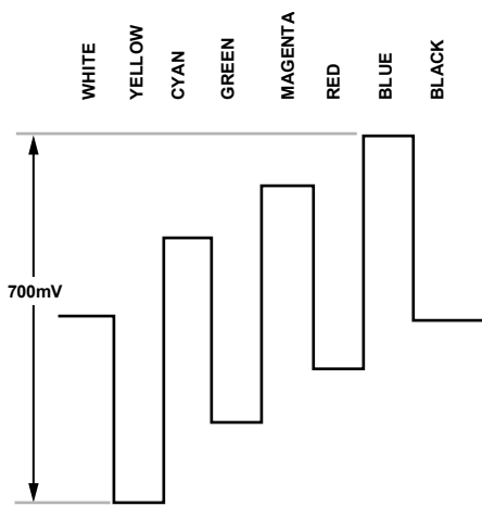
Figure 117. Pb Levels—NTSC
