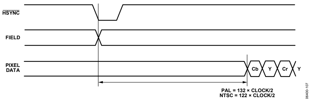
Figure 107. SD Timing Mode 1, Odd/Even Field Transitions (Master/Slave)
