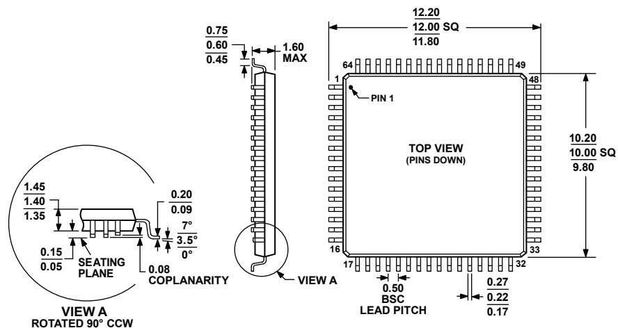
Figure 141. 64-Lead Low Profile Quad Flat Package [LQFP] (ST-64-2)
