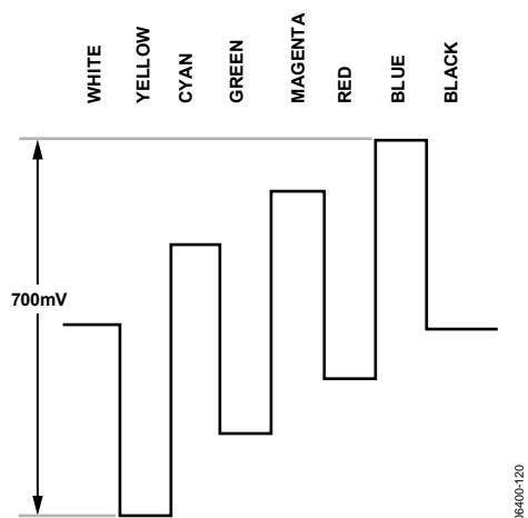
Figure 120. Pb Levels—PAL
