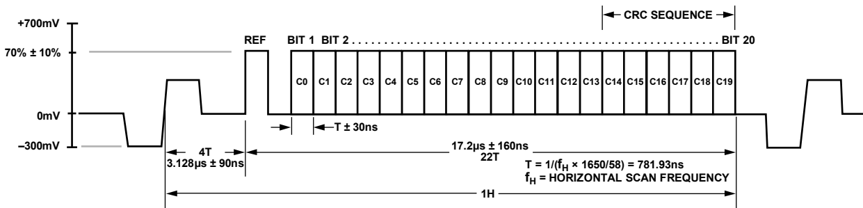
Figure 95. High Definition (720p) CGMS Waveform
