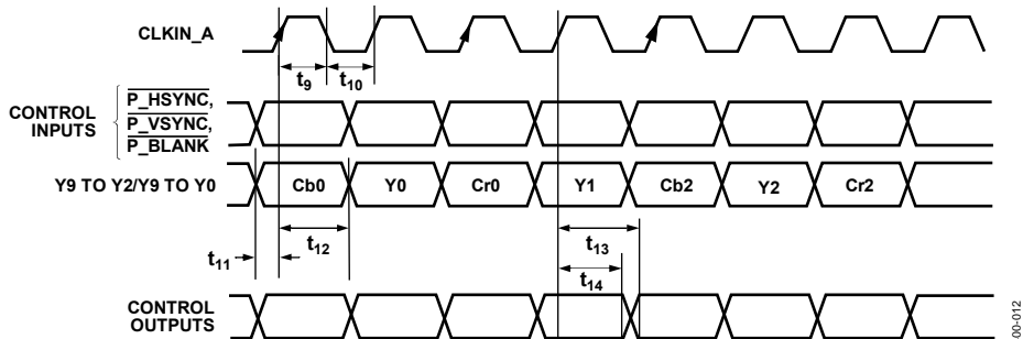
Figure 12. ED Only (at 54 MHz), 8-/10-Bit, 4:2:2 YCrCb (HSYNC/VSYNC) Pixel Input Mode (Input Mode 111)
