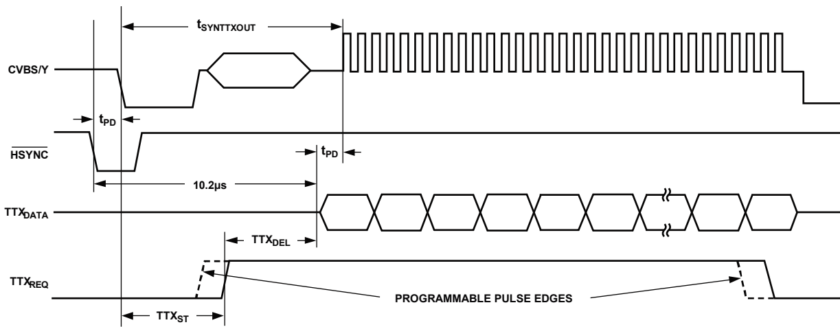
Figure 83. Teletext VBI Line
