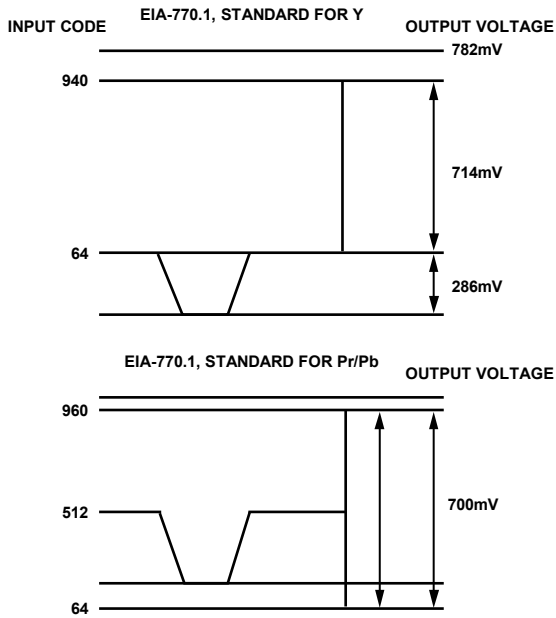
Figure 122. EIA-770.1 Standard Output Signals (525p/625p)
