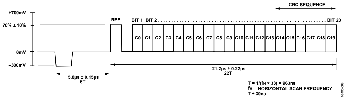
Figure 93. Enhanced Definition (525p) CGMS Waveform
