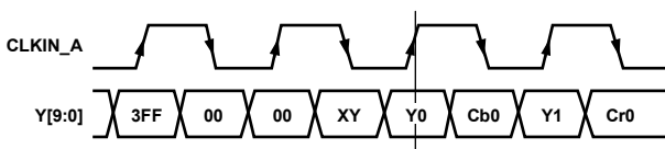
Figure 51. ED/HD-DDR Input Sequence (EAV/SAV)—Option A
