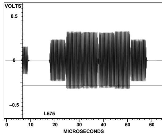
Figure 133. PAL Luma
