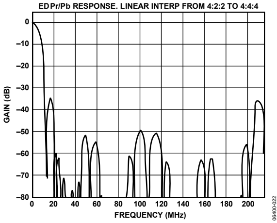
Figure 21. ED 8× Oversampling, Pr/Pb Filter (Linear) Response
