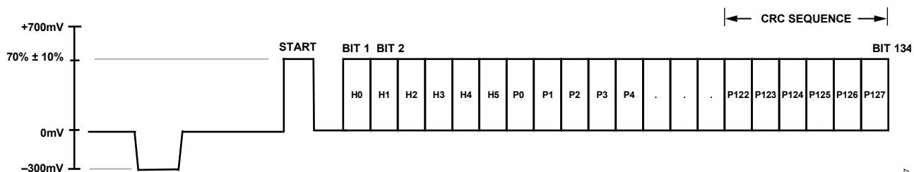
Figure 97. Enhanced Definition (525p) CGMS Type B Waveform
