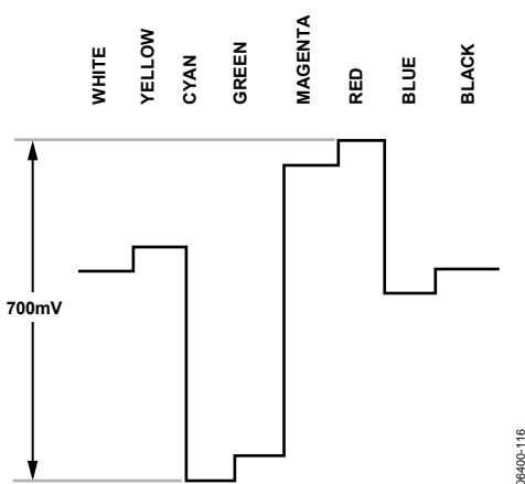
Figure 116. Pr Levels—NTSC
