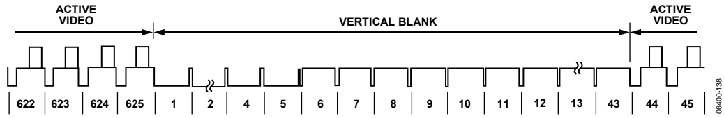
Figure 138. ITU-R BT.1358 (625p)
