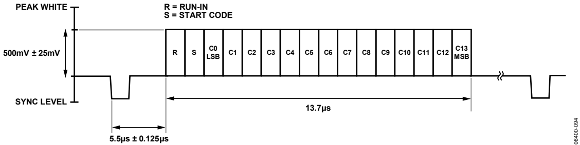
Figure 94. Enhanced Definition (625p) CGMS Waveform
