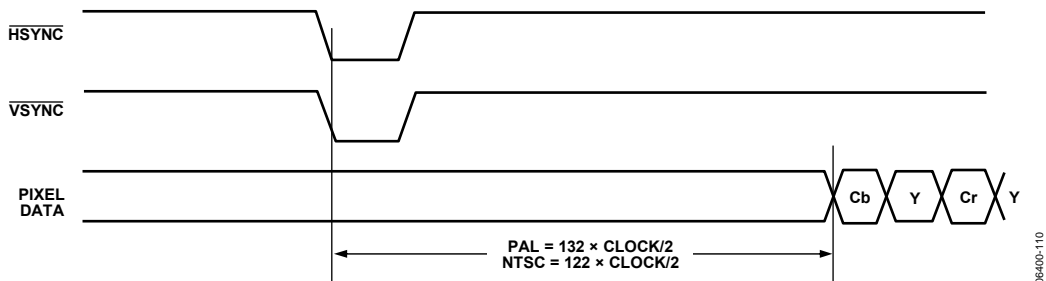
Figure 110. SD Timing Mode 2, Even-to-Odd Field Transition (Master/Slave)
