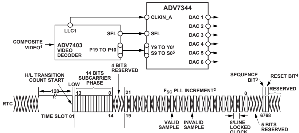
Figure 60. SD Subcarrier Phase Reset Timing Diagram (Subaddress 0x84, Bits[2:1] = 01)
