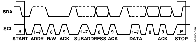
Figure 48. I 2 C Data Transfer
