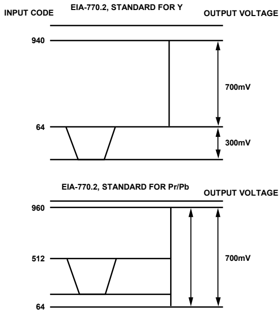
Figure 121. EIA-770.2 Standard Output Signals (525p/625p)
