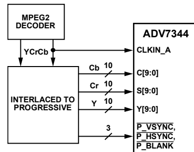
Figure 53. ED/HD Only Example Application
