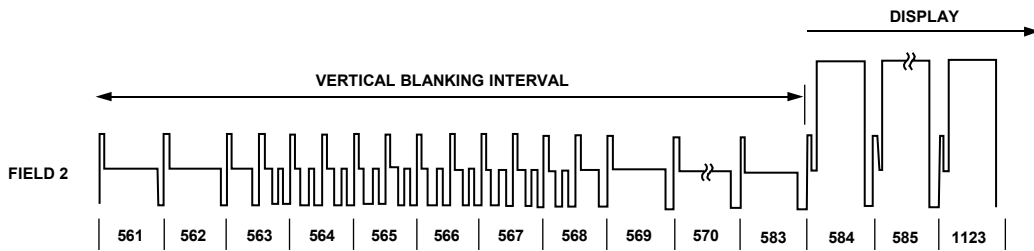
Figure 140. SMPTE 274M (1080i)
