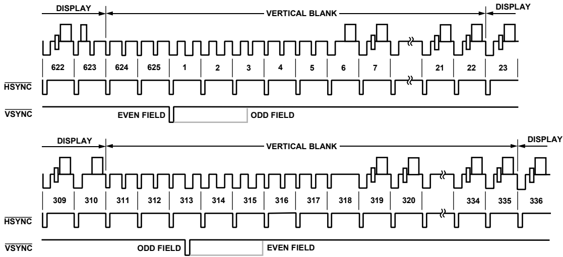
Figure 109. SD Slave Mode 2, PAL
