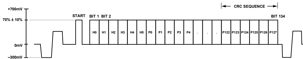
Figure 98. High Definition (720p and 1080i) CGMS Type B Waveform
