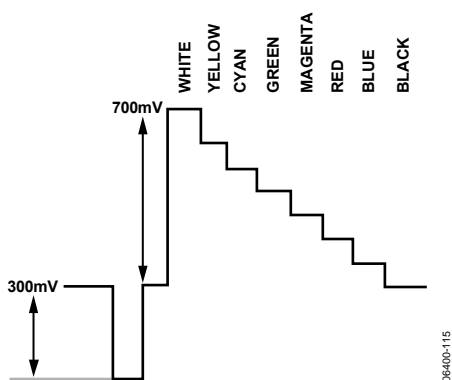
Figure 115. Y Levels—NTSC
