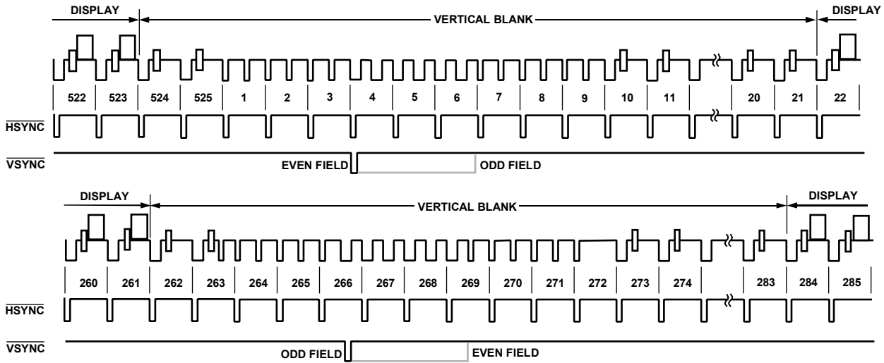
Figure 108. SD Slave Mode 2, NTSC
