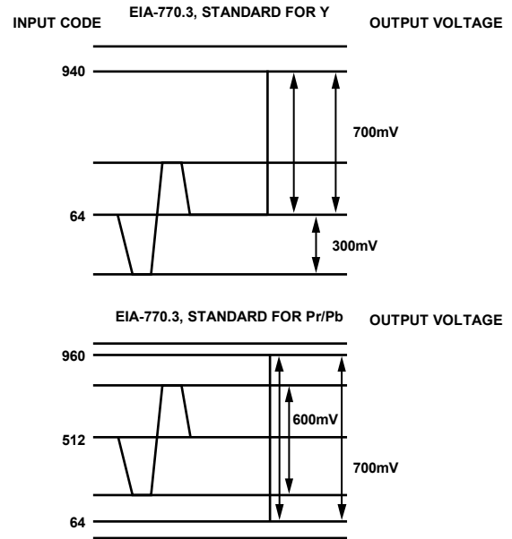
Figure 123. EIA-770.3 Standard Output Signals (1080i/720p)
