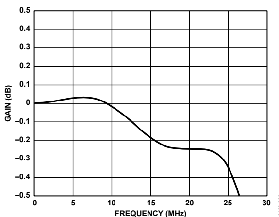
Figure 66. ED/HD Sinc Compensation Filter Disabled
