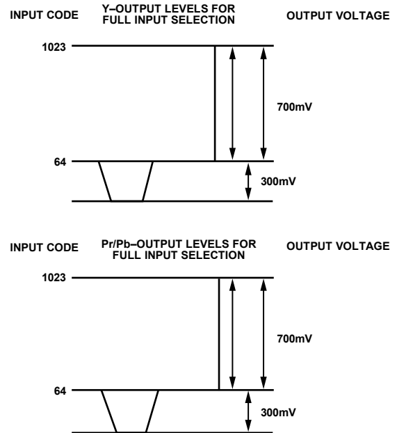
Figure 124. Output Levels for Full Input Selection
