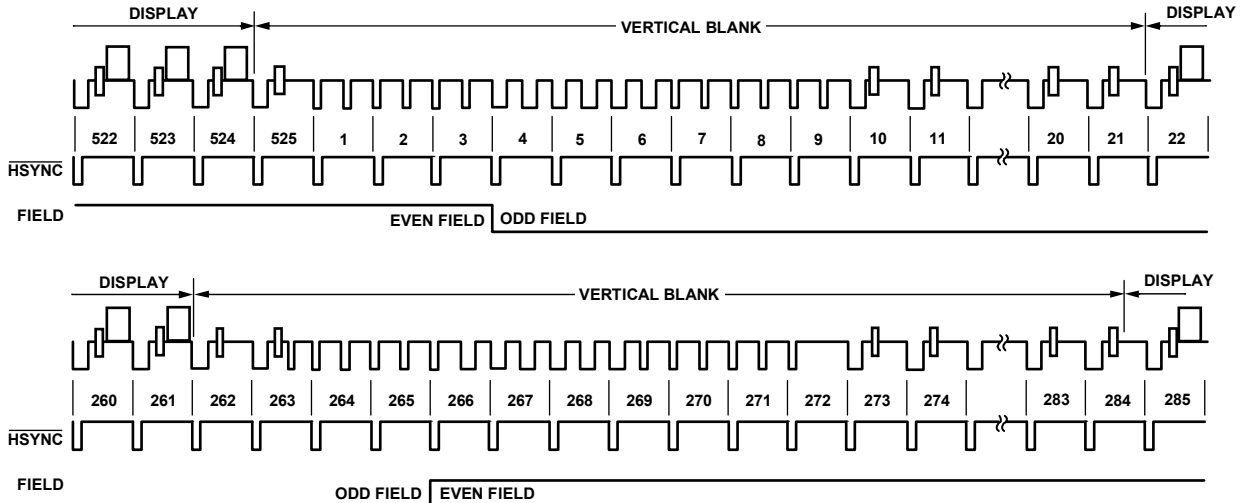
Figure 105. SD Slave Mode 1, NTSC
