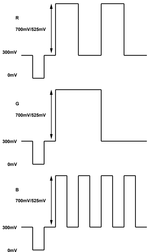
Figure 126. SD/ED RGB Output Levels—RGB Sync Enabled
