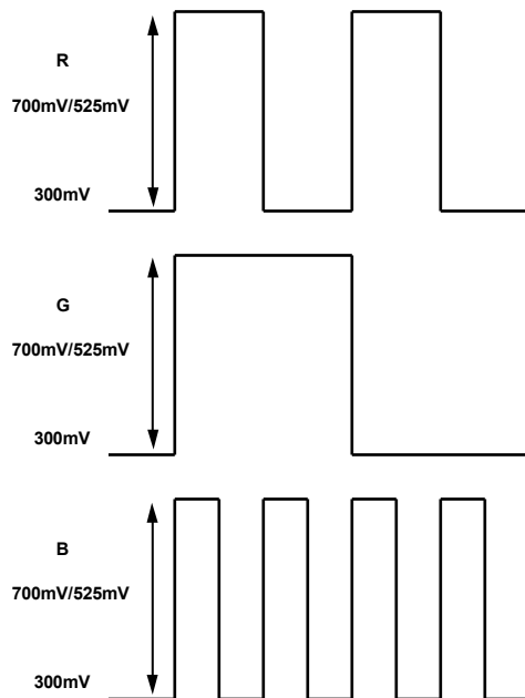
Figure 127. HD RGB Output Levels—RGB Sync Disabled
