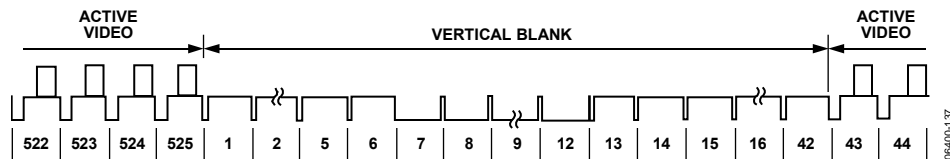
Figure 137. SMPTE 293M (525p)
