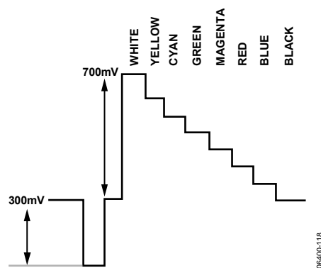
Figure 118. Y Levels—PAL
