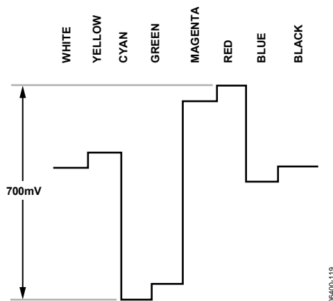
Figure 119. Pr Levels—PAL
