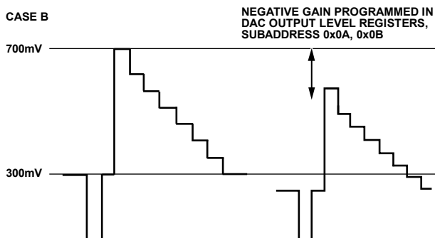
Figure 68. Programmable DAC Gain—Positive and Negative Gain
