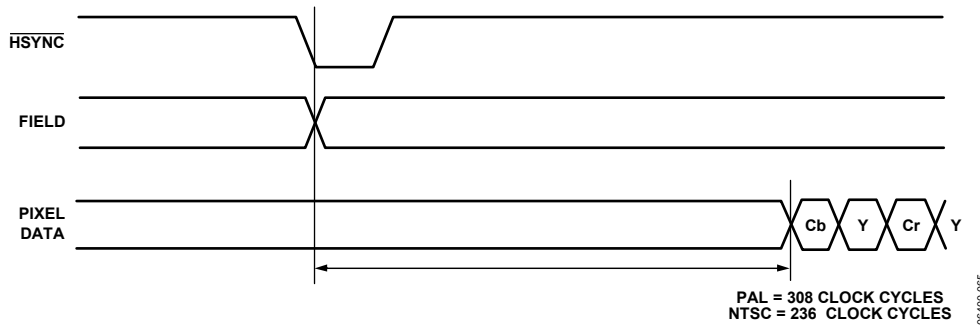
Figure 63. Square Pixel Mode Active Pixel Timing
