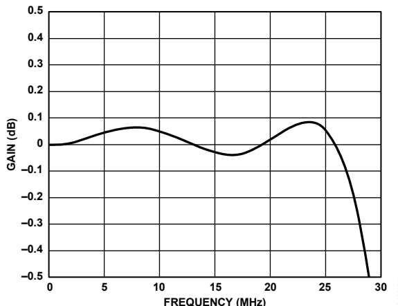
Figure 65. ED/HD Sinc Compensation Filter Enabled
