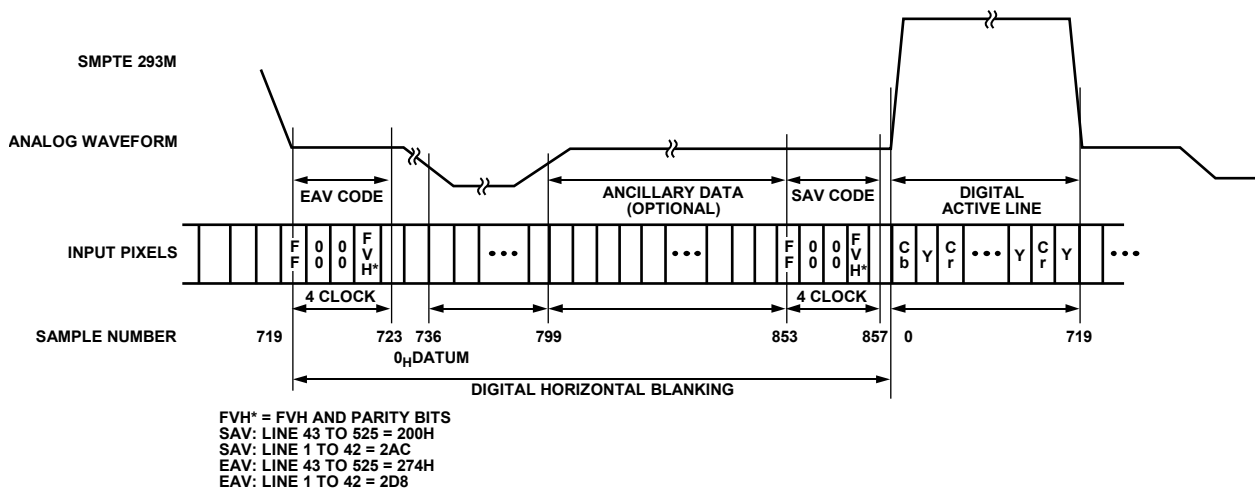
Figure 136. EAV/SAV Input Data Timing Diagram (SMPTE 293M)
