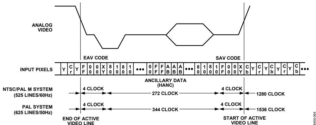
Figure 62. Square Pixel Mode EAV/SAV Embedded Timing
