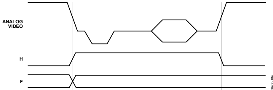
Figure 104. SD Master Mode 0, Data Transitions
